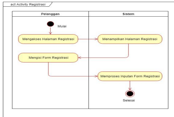
Gambar 2. Activity Diagram
